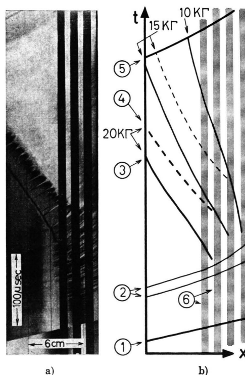
Fig. 2. Streak interferogram at 20 kG, and graphic representation of the reflected-shock-path dependence on magnetic field strength; M_s=9.6 , P_0=10 torr. The various lines indicate: 1) primary shock, 2) particle paths, 3) reflected shock, 4) ionization front, 5) contact front, 6) electrode short circuit bridges.
